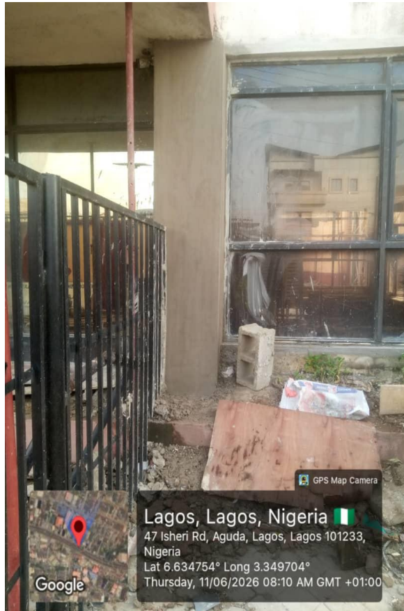
Jacketed Column on the 5-storey JAMB Building at Ogba, Ikeja, Lagos
